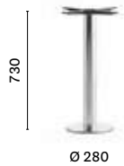
COLUMN Ø 76 TOP MAX 900x900; Ø1100
