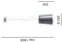
L001S/AA* (A+A) Suspension lamp with two polycarbonate diffusers
